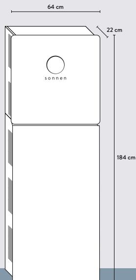
eco 8.0/2 - 8.0/16 Usable battery capacity: 2,0-16,0 kWh
