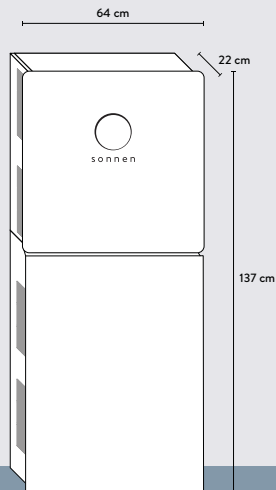
eco 8.0/2 - 8.0/10 Usable battery capacity: 2,0-10,0 kWh
